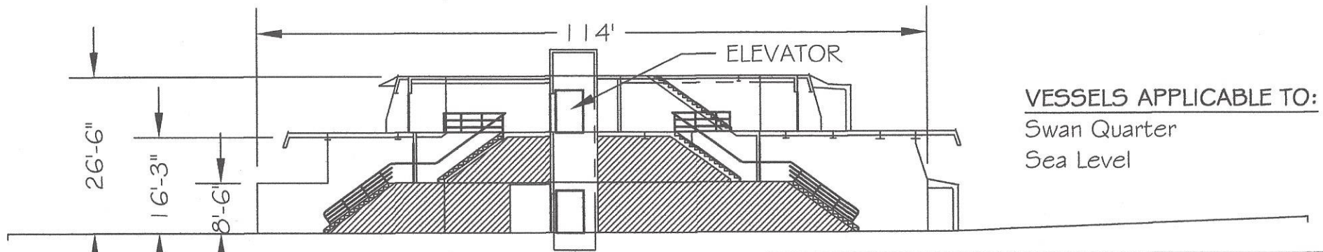
INBOARD PROFILE
