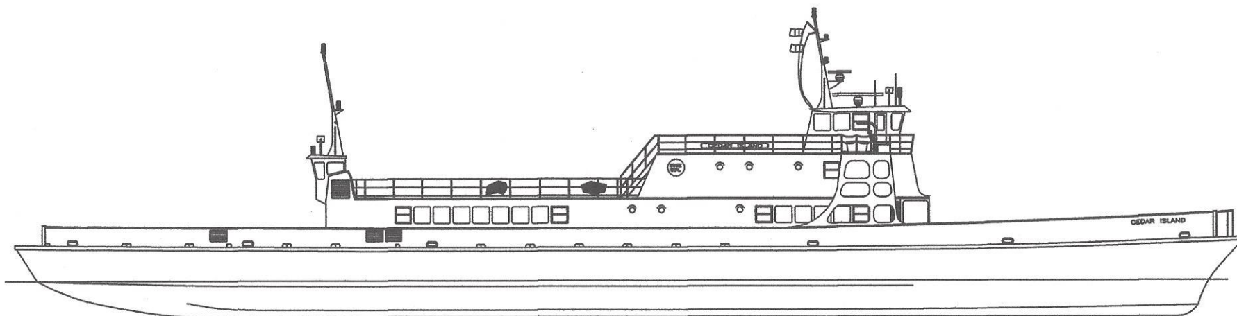
OUTBOARD PROFILE STBD SIDE SHOWN, PORT SIM
