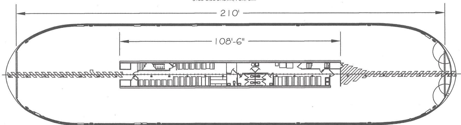
MAIN DECK ARRANGEMENT
